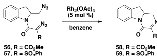
Scheme 4.11: First example of Rh-catalyzed reaction of an azide with a metallocarbenes.
