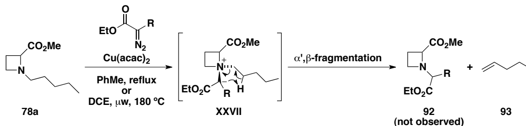
Scheme 2.16: Possible \alpha',\beta -fragmentation pathway of N-pentyl azetidine 78a
