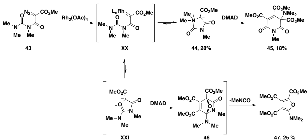
Scheme 4.8: Insight into ylide equilibrium in the presence of DMAD.
