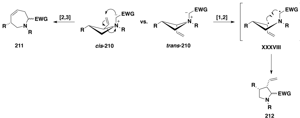
Scheme 1.64: Explanation for observed reactivity of cis and trans 2-alkenylazetidines.
