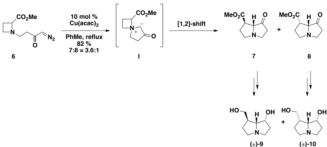
Scheme 3.3: Synthesis of the pyrrolizidine alkaloids turneforicidine and platynecine.
