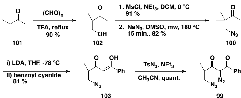
Scheme 4.25: Synthesis of an acyclic diazo-azide substrate.
