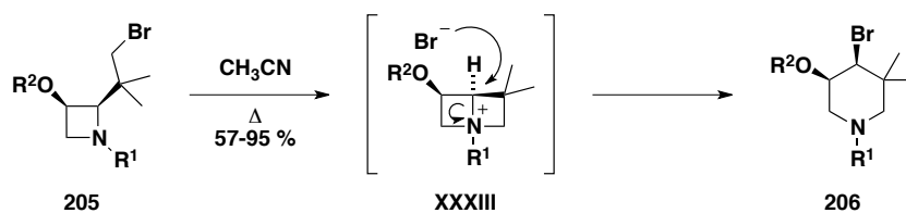
Scheme 1.61: Ring expansion of azetidines to piperidines.
