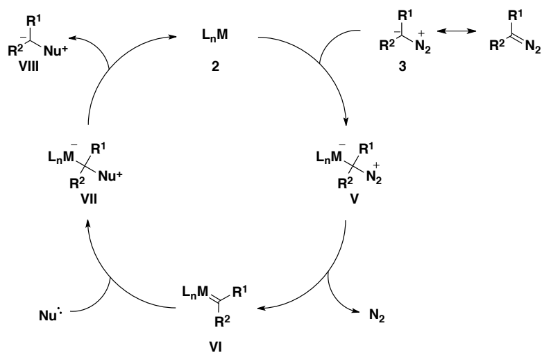
Scheme 4.2: Mechanism of ylide generation via metalcarbenes.
