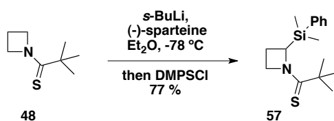
Scheme 3.21: Synthesis of the \alpha -DMPS-azetidine derivative 57 .
