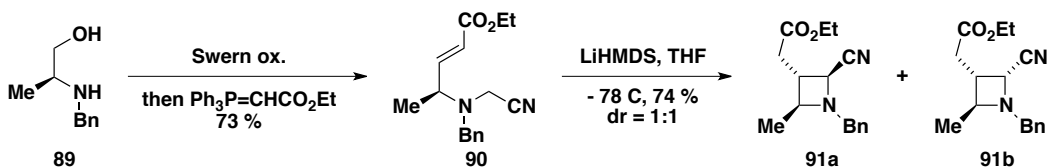
Scheme 1.16: The application of Michael addition towards azetidine synthesis.
