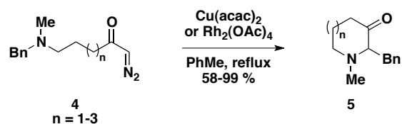
Scheme 3.2: Synthesis of aza-heterocycles via an intramolecular Stevens [1,2]-shift.
