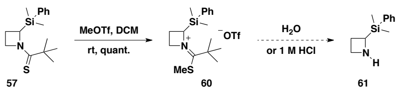
Scheme 3.23: Synthesis of a stable thioimidate salt from azetidine 57 .
