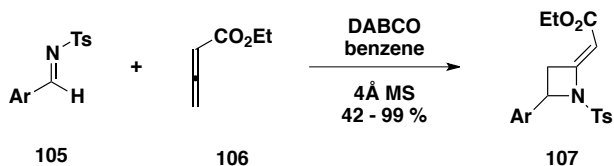
Scheme 1.22: Azetidine formation under Baylis-Hillman conditions.
