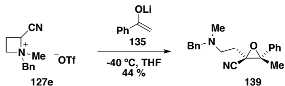
Scheme 1.38: Unexpected epoxide formation.
