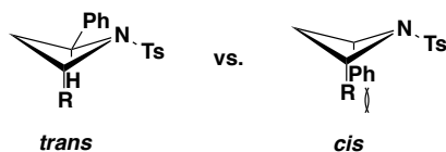
Figure 1.5: Comparison of steric interactions in cis and trans -2,4-disubstituted azetidines.
