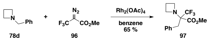
Scheme 2.20: Example of benzyl [1,2]-shift by Burger and coworkers.
