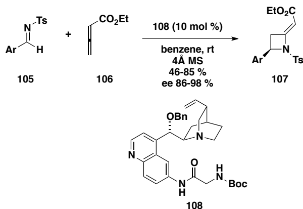
Scheme 1.23: Asymmetric synthesis of azetidines using a cinchona alkaloid catalyst.
