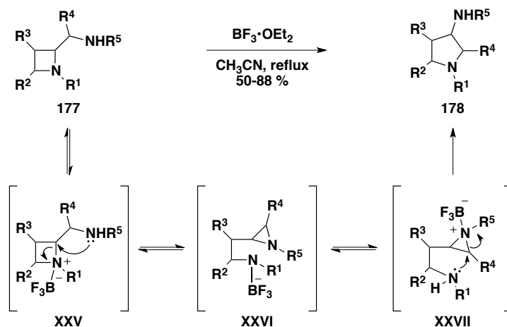
Scheme 1.53: Lewis acid activated ring expansion of \alpha -aminomethyl azetidines.
