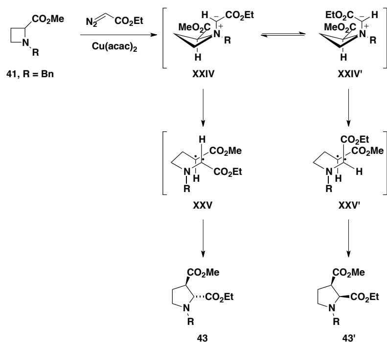
Scheme 2.14: Mechanistic rationale for the formation of diastereomers.
