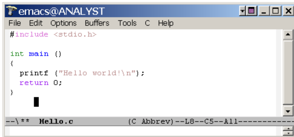
Figure 8. An Emacs frame displaying the file Hello.c , which contains C source code for a classical “Hello world” program. The frame includes a title bar, menu bar, editing window, status line, and echo area (or minibuffer window). Emacs recognises the .c file extension and highlights text in a manner consistent with C code. The black rectangular cursor lies in line 8 to the right of column 5 (L8–C5 in the status line).
