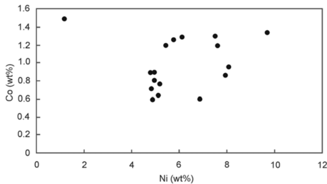
Fig. 10. Variation in cobalt and nickel composition among native iron metal grains in SaU 300. Most analyzed grains fall within the range of meteoritic metal as defined by Hewins and Goldstein (1975). This composition is common in lunar feldspathic impact melt rocks (Papike et al. 1998).
