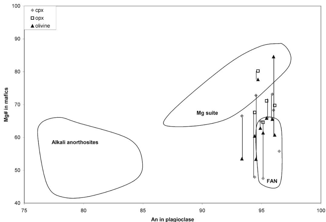
Fig. 12. Mg# (molar \text{Mg}/[\text{Mg} + \text{Fe}] \times 100 ) in mafic minerals (olivine and pyroxene) versus An (molar \text{Ca}/[\text{Ca} + \text{Na} + \text{K}] \times 100 ) in feldspars for minerals present in the lithic clasts observed in SaU 300. Fields are for the pristine rock suites (Warren et al. 1983). FAN = ferroan anorthosite suite.
