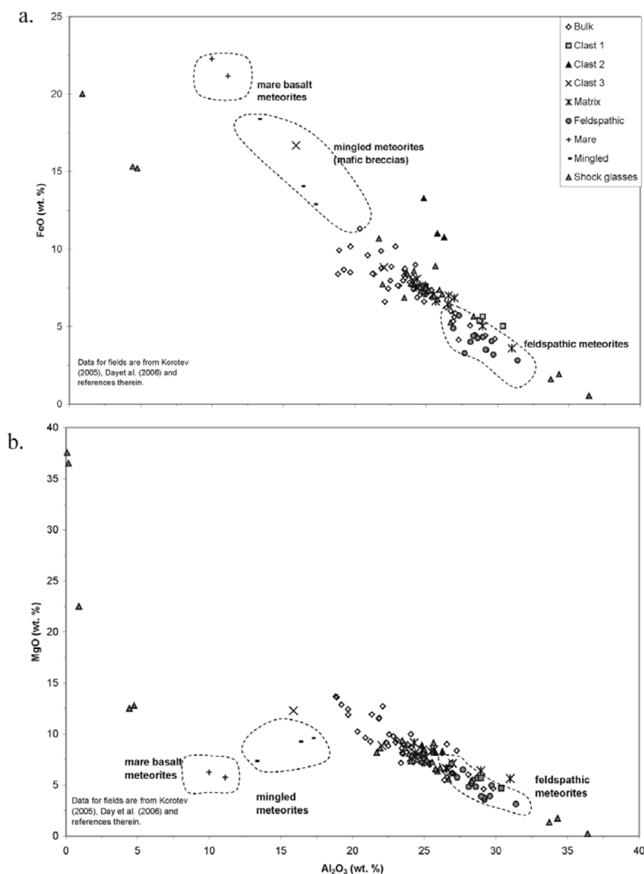
Fig. 11. Plot of \text{Al}_2\text{O}_3 (in weight percent) versus (a) FeO and (b) MgO. Included are whole rock, matrix, lithic clast, glass, and shock melt compositions for SaU 300. These have been plotted against the compositions of a range of other meteorites taken from the literature (data from Korotev [2005], Day et al. [2006] and references therein).
