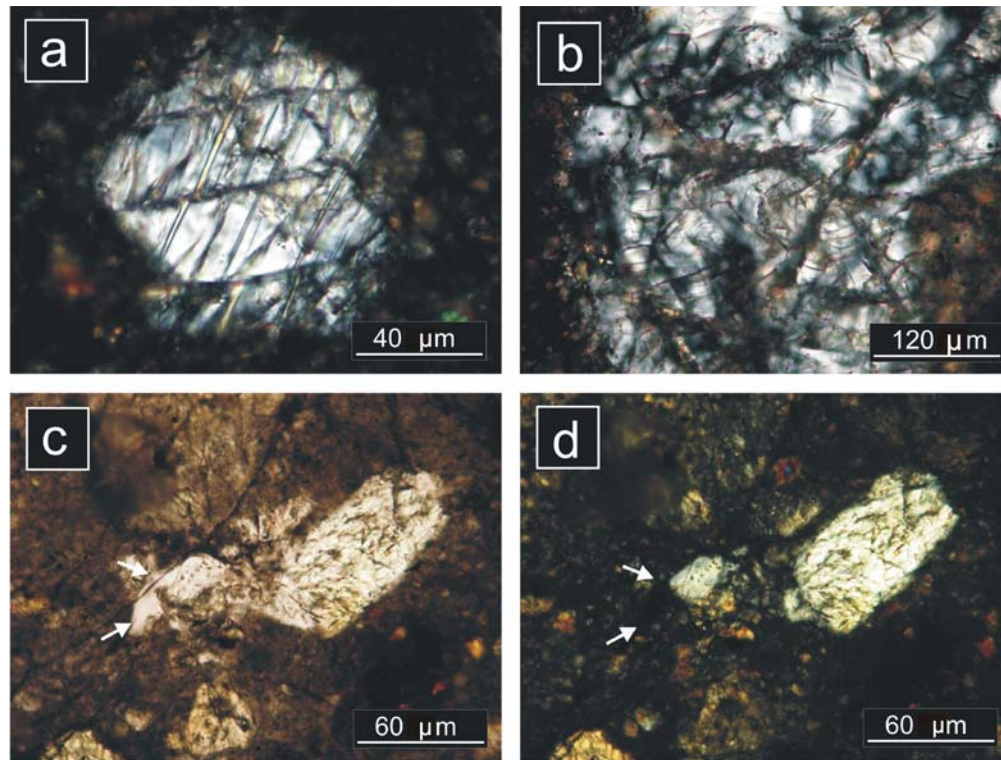
Fig. 6. Optical photomicrographs of SaU 300 anorthite in thin section. a) Anorthite mineral fragment showing mechanical deformation (offsetting of twin planes). b) Internally brecciated anorthite clast with patchy maskelynitization. c) Plane-light view of anorthite clast cut by shock vein (thin dark vein) as indicated by arrows. d) Cross-polarized image of (c). The anorthite devoid of fractures is optically isotropic.
