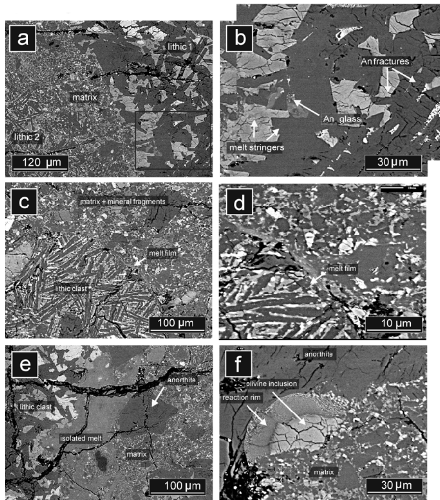
Fig. 2. BSE images of margins between matrix and lithic clasts. a) Overview of matrix-lithic clast relations. b) Close-up of area outlined in (a) showing isolated stringers and pockets of silicate melt near the clast margin. Anorthite, with irregular fractures and 1^\circ birefringence throughout, has been transformed to glass near the matrix contact. Light areas are pyroxene grains. c) A thin film of melt occurs at a clast/matrix contact. d) Close-up of (c). e) An isolated pocket of silicate melt occurs at the margin between clast and matrix. f) Broken edge of lithic clast with olivine- (core) reaction rim inclusion set within anorthite host clast, juxtaposed with matrix.
