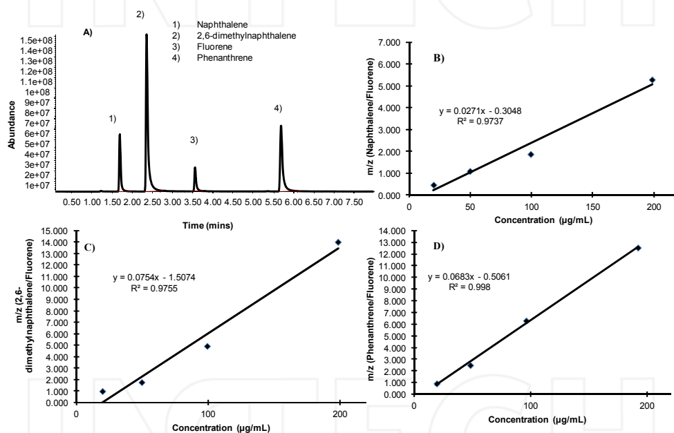
Fig. 6. A) GC-MS chromatogram showing separation of 100 \mu\text{g/mL} of three PAHs including; 1) naphthalene, 2) 2,6-dimethylnaphthalene, 3) fluorene, and 4) phenanthrene extracted by poly(Styrene-co-DVB) PPME; Calibration curves of B) naphthalene; C) 2,6-dimethylnaphthalene; D) phenanthrene extracted by poly(Styrene-co-DVB) PPME with 30 second adsorption and fluorene as an internal standard.
