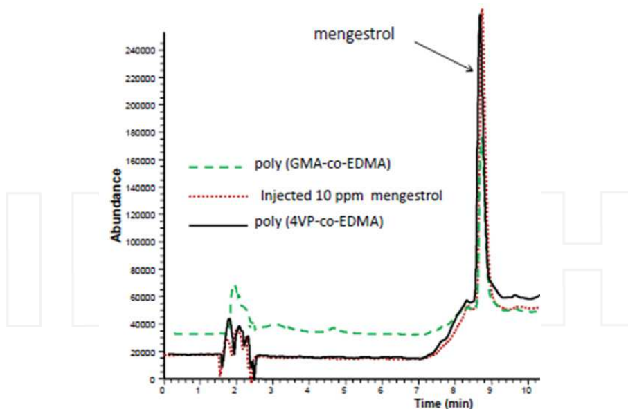
Fig. 8. Overlapped chromatogram indicating meggestrol peak for poly( 4VP-co-EDMA) and poly (GMA-co-EDMA) and directly injected 10 ppm meggestrol standard.
